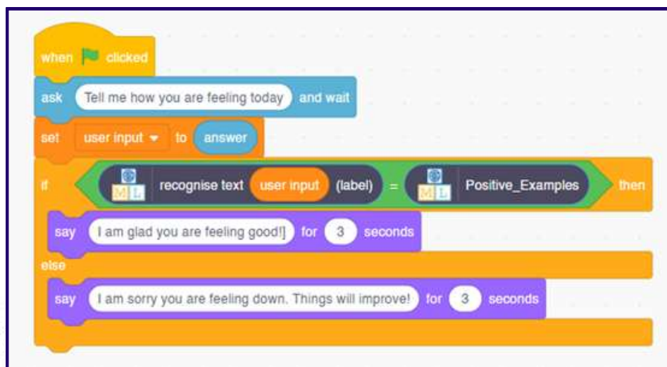
Abb. 4 Sequence of code blocks in Scratch illustrating a basic event-action chain: Scratch by MIT Media Lab
