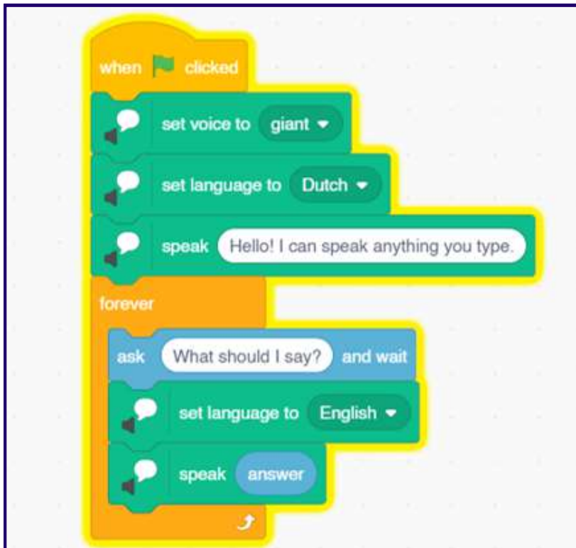
Abb. 6 Sequence of code blocks in Scratch: Scratch by MIT Media Lab
